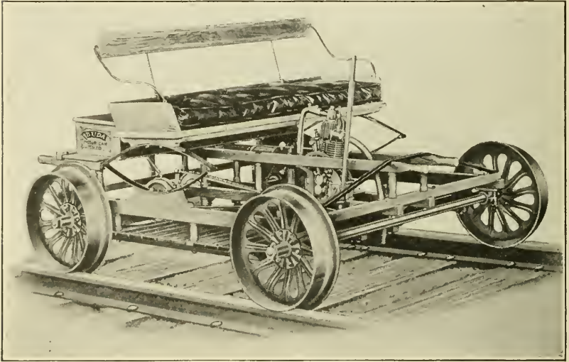
Fig. 2. Inspection Motor Car.
